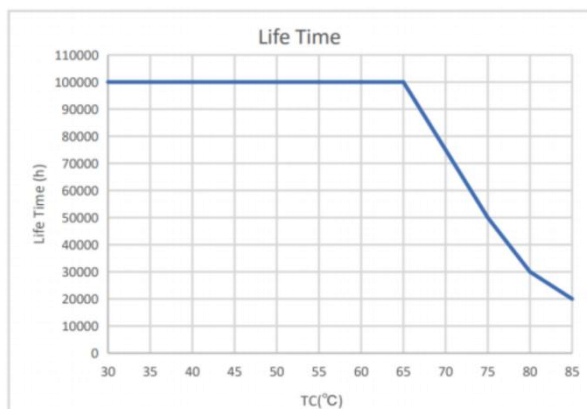
Lifetime vs. Temperature Curve
